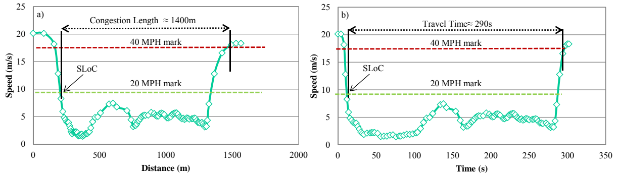
Figure 4-3: (a) The Vehicle Speed Through the Congestion vs. Relative Distance. (b) The Same Speed vs. Time.
