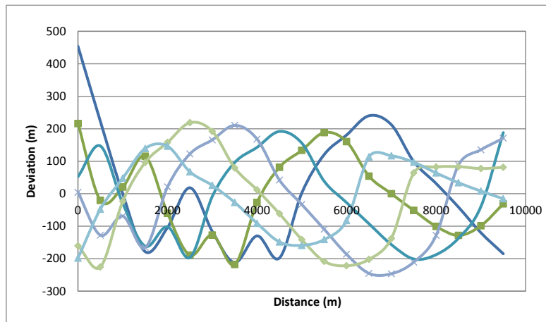
Figure 2-2: The Deviation of the Polynomial Fit Calculated Distance from the Actual Road Distance. Different Colors are for Multiple Road Segments.
