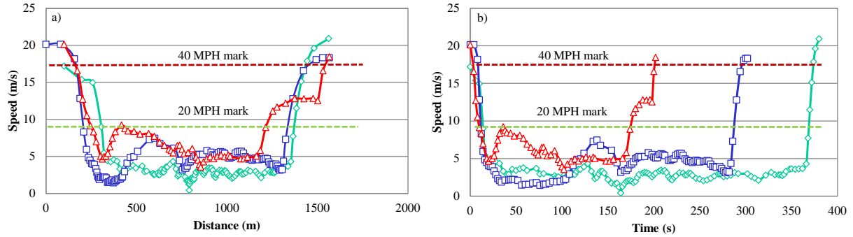
Figure 4-4: The Vehicle Speed Through the Congestion vs. Relative Distance and Time for Different Congestion Behaviors. Different Colors are for Different Test Trials.
