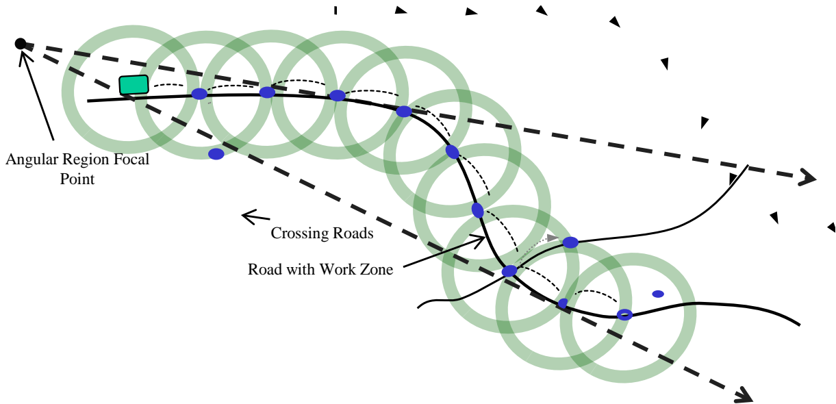
Figure 3-3: Directional Relay Functionality of V2V-Assisted V2I Communication Protocol.
