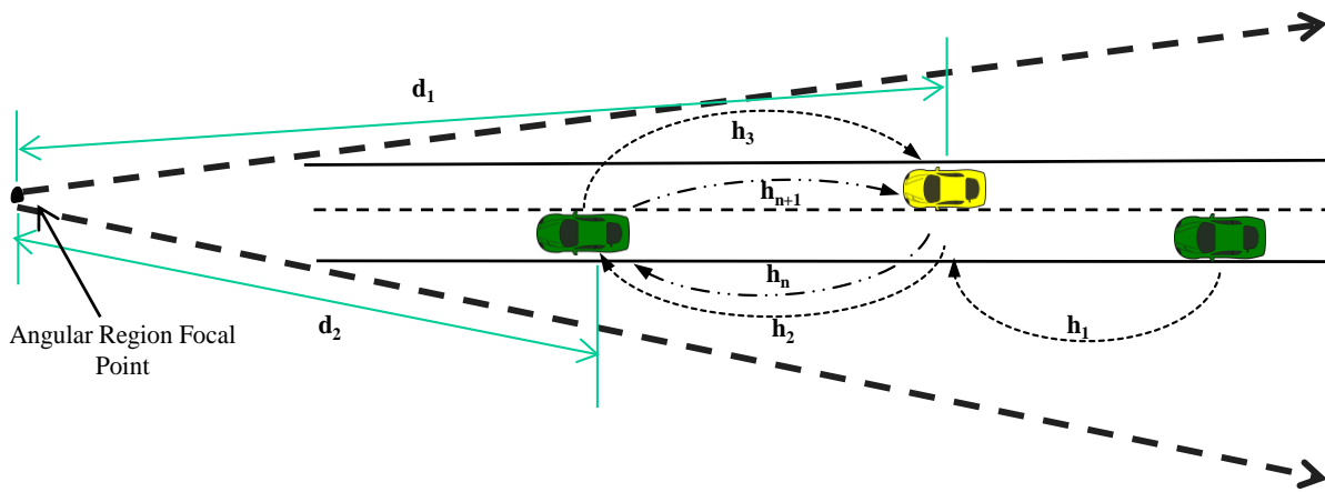
Figure 3-4: Conceptual Diagram Showing Handling of Message Back Propagation in V2V-Assisted V2I Communication Protocol.
